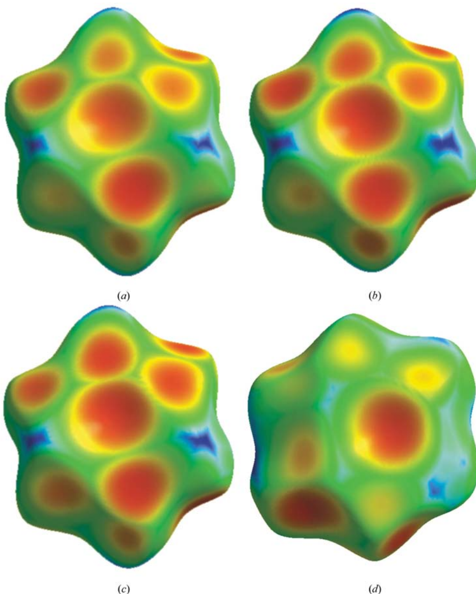
Figure 8 The interactions of the benzene molecule represented as a colour scale on the Hirshfeld surface at 296 K: (a) in phase I at 0.3 GPa; (b) 0.7 GPa; (c) 1.1 GPa; (d) in phase III at 2.5 GPa.
