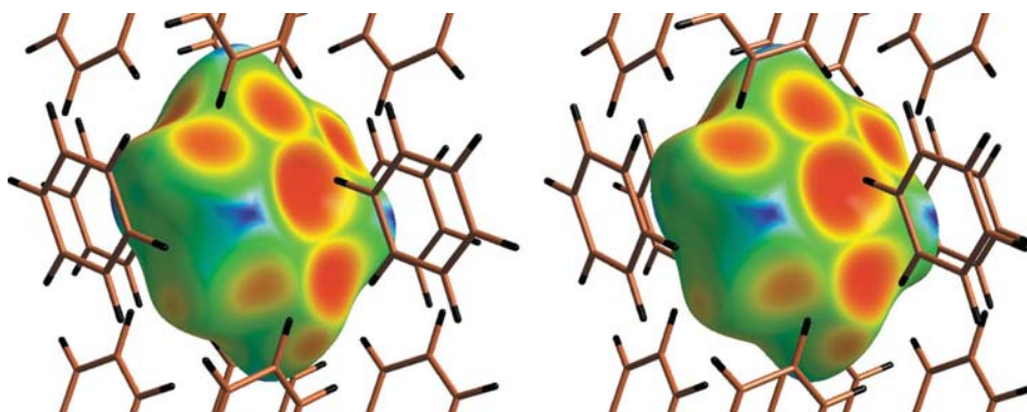
Figure 7 A stereoscopic view of one benzene molecule in phase I at 138 K and 0.1 MPa represented as a Hirshfeld surface. The colour scale on the Hirshfeld surface represents the close intermolecular distances (red for the shortest, blue for the longest). The crystal [010] axis is vertical in this drawing and the viewing direction is at ca 30 and 60° to the [100] and [001] axes, respectively.
