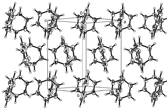
Figure 6 Autostereogram (Katrusiak, 2001 a,b ) of the benzene I structure at 0.7 GPa viewed down [101]. The thermal ellipsoids have been drawn at the 50% probability level, and the H atoms have been shown as spheres of arbitrary radius.
