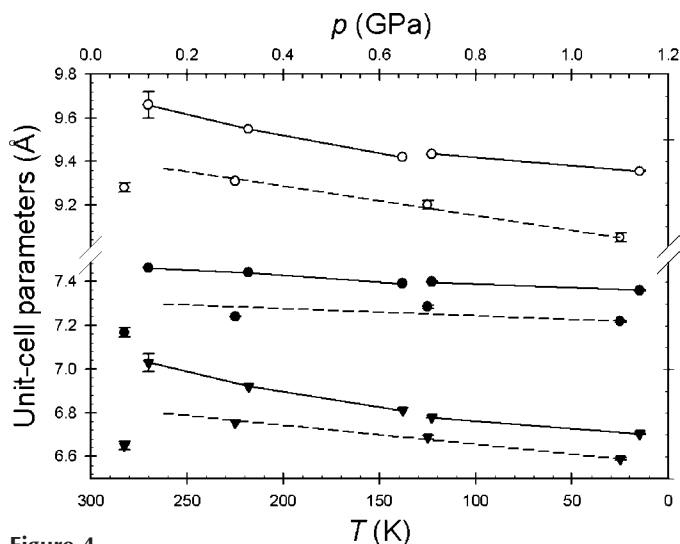
Figure 4 Unit-cell dimensions of benzene I plotted as a function of pressure (shown as dashed lines; the scale in GPa units is at the top of the plot) and as a function of temperature (the reverse scale at the bottom and solid-line plots). Low-temperature data were measured for C 6 H 6 (Cox et al. , 1958; Bacon et al. , 1964) and C 6 D 6 at 123 and 15 K (Jeffrey et al. , 1987). The unit-cell parameters measured at 0.07 GPa (Weir et al. , 1969) have been excluded from the regression lines, as they considerably divert from the other results – see the text.
