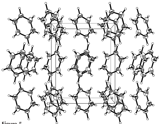
Figure 5 Autostereogram (Katrusiak, 2001 a,b ) of the benzene I structure at 0.7 GPa viewed down [001]. The thermal ellipsoids have been drawn at the 50% probability level, and the H atoms have been shown as spheres of arbitrary radius.
