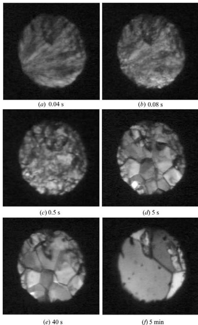
Figure 2 Benzene pressure-frozen in phase I at (a) 296 K and 0.07 GPa, and (b)–(f) the time evolution of the spontaneous re-crystallization process inside the DAC at 296 K and 0.07 GPa. The time-lapses from the moment of freezing are given below the photographs.
