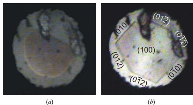
Figure 3 Two characteristic morphologies of the benzene crystals in phase I: (a) the globular single crystal at \sim 0.3 GPa and 310 K; (b) a single crystal with well developed faces at about 400 K, growing at isochoric conditions in the DAC after benzene was pressure-frozen at ca 100 MPa at room temperature and then heated to melting, except for one grain. Two ruby chips for pressure calibration are visible at the top and right edges of the DAC chamber.
